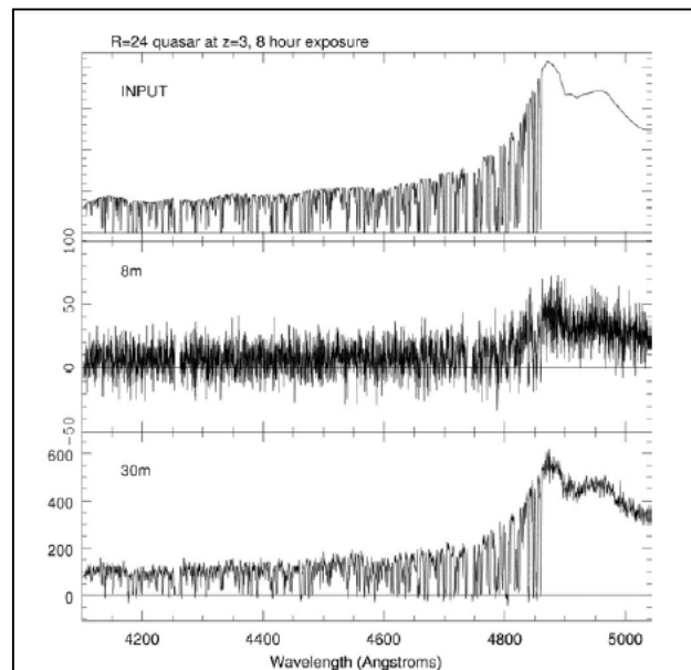
Figure 2. A plot depicting a simulation of the "forest" of hydrogen and metal absorption lines as they might appear observed against the spectrum of a faint quasar (top). The middle spectrum reveals the best result we could expect for today's 8–10-m diameter telescopes, even with an all-night exposure. The bottom spectrum illustrates the potential of the TMT to deliver spectra capable of analyzing these absorption features and deducing the distribution, chemical composition, and motions of intergalactic gas. To gather the million-galaxy sample capable of providing a tomographic map of the intergalactic medium will require nearly two full years of observation, even with the TMT. Simulation courtesy: J. Bechtold (U. Arizona).
